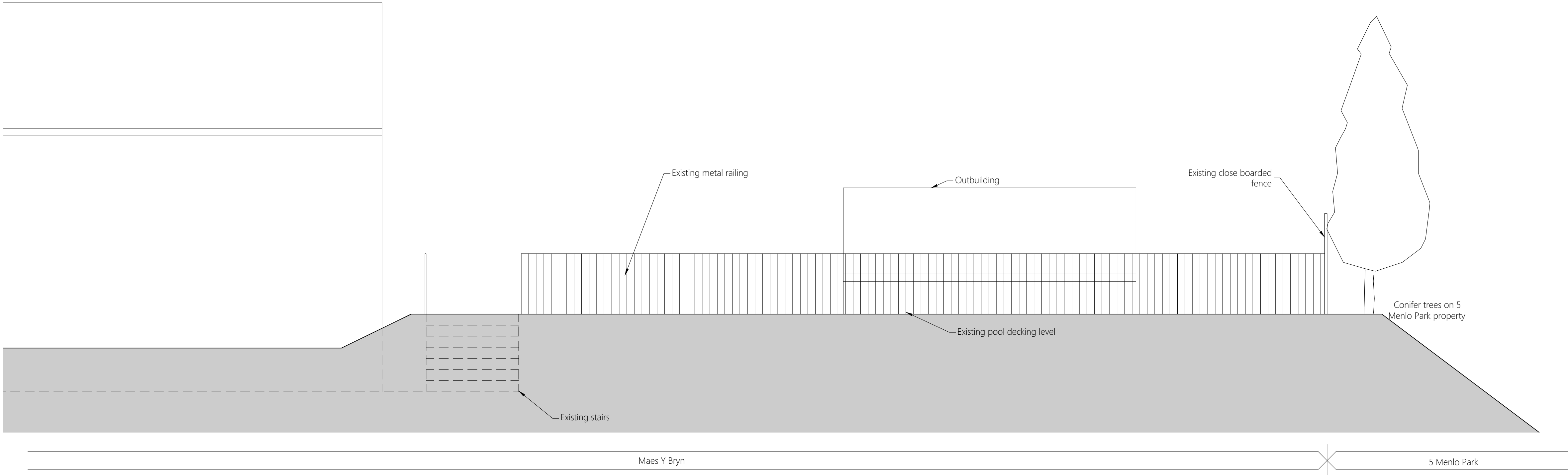
1 Existing Site Section 4 0403 1:50 @ A1
