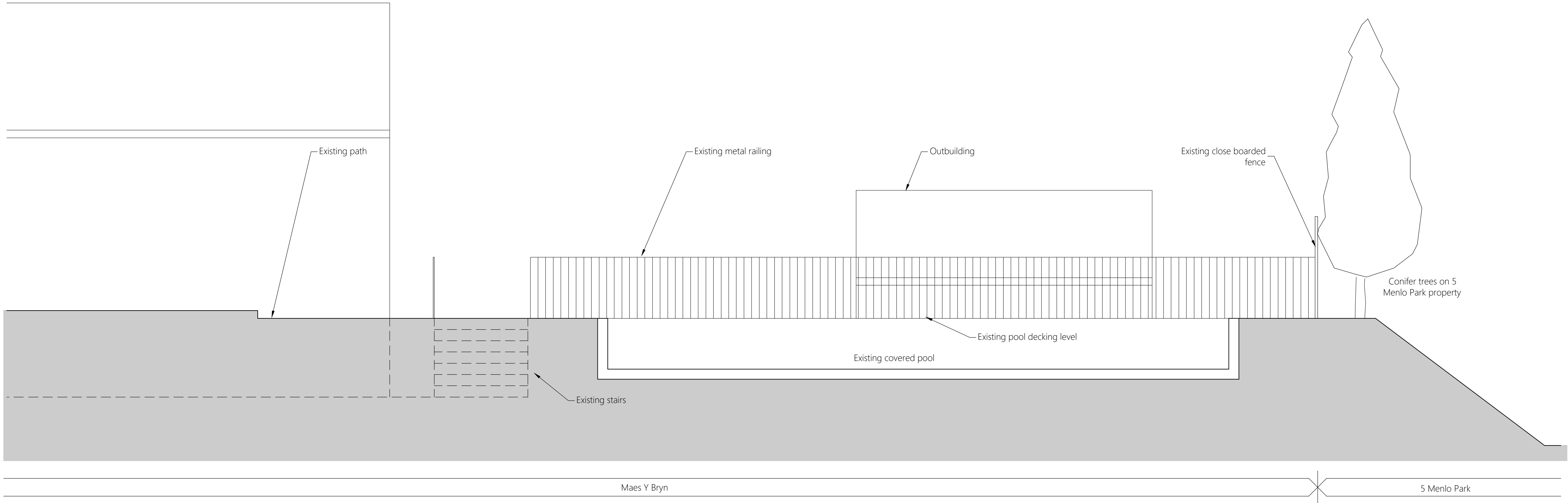
1 Existing Site Section 3 0402 1:50 @ A1
