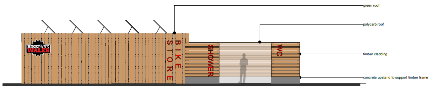
FRONT ELEVATION
