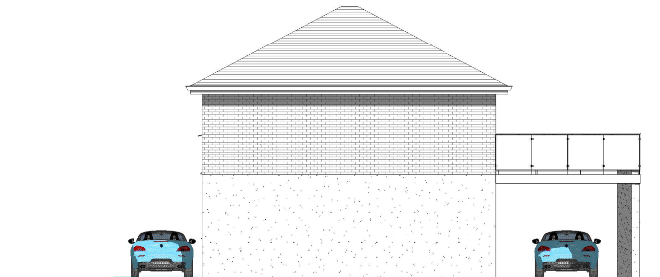
2 Proposed Rear Elevation 1 : 100
