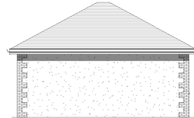
5 Existing Side 1 Elevation 1 : 100
