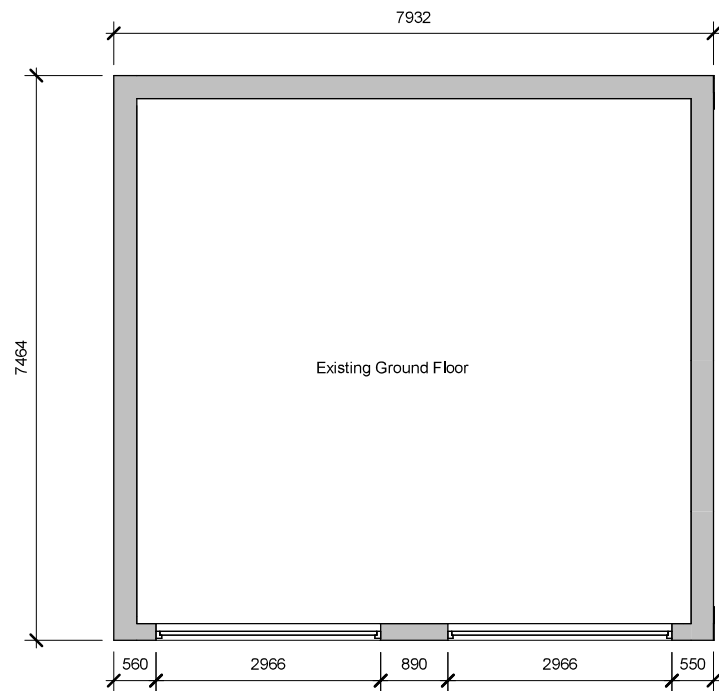
1 Existing Ground Floor 1 : 100
