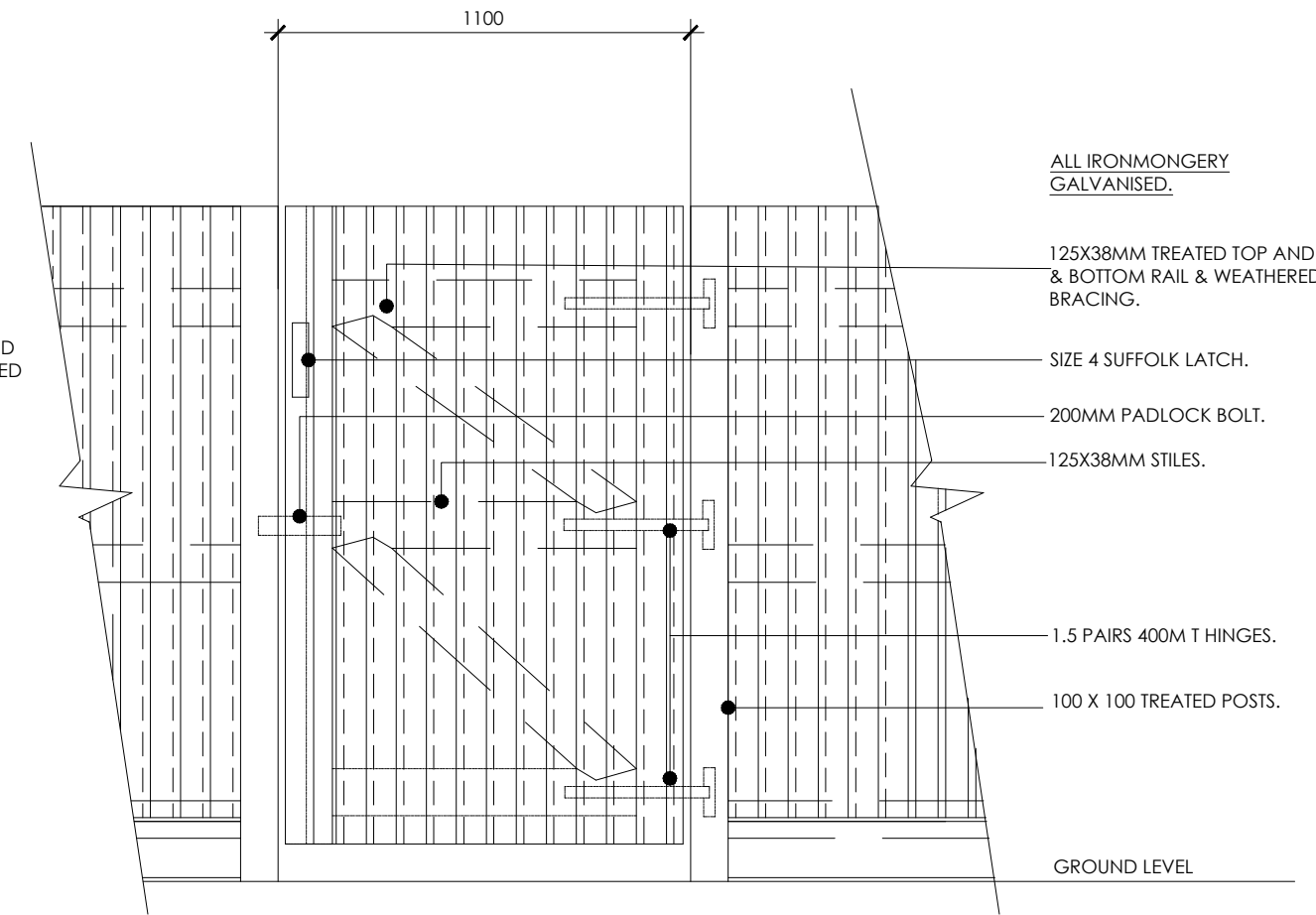
OUTSIDE ELEVATION
