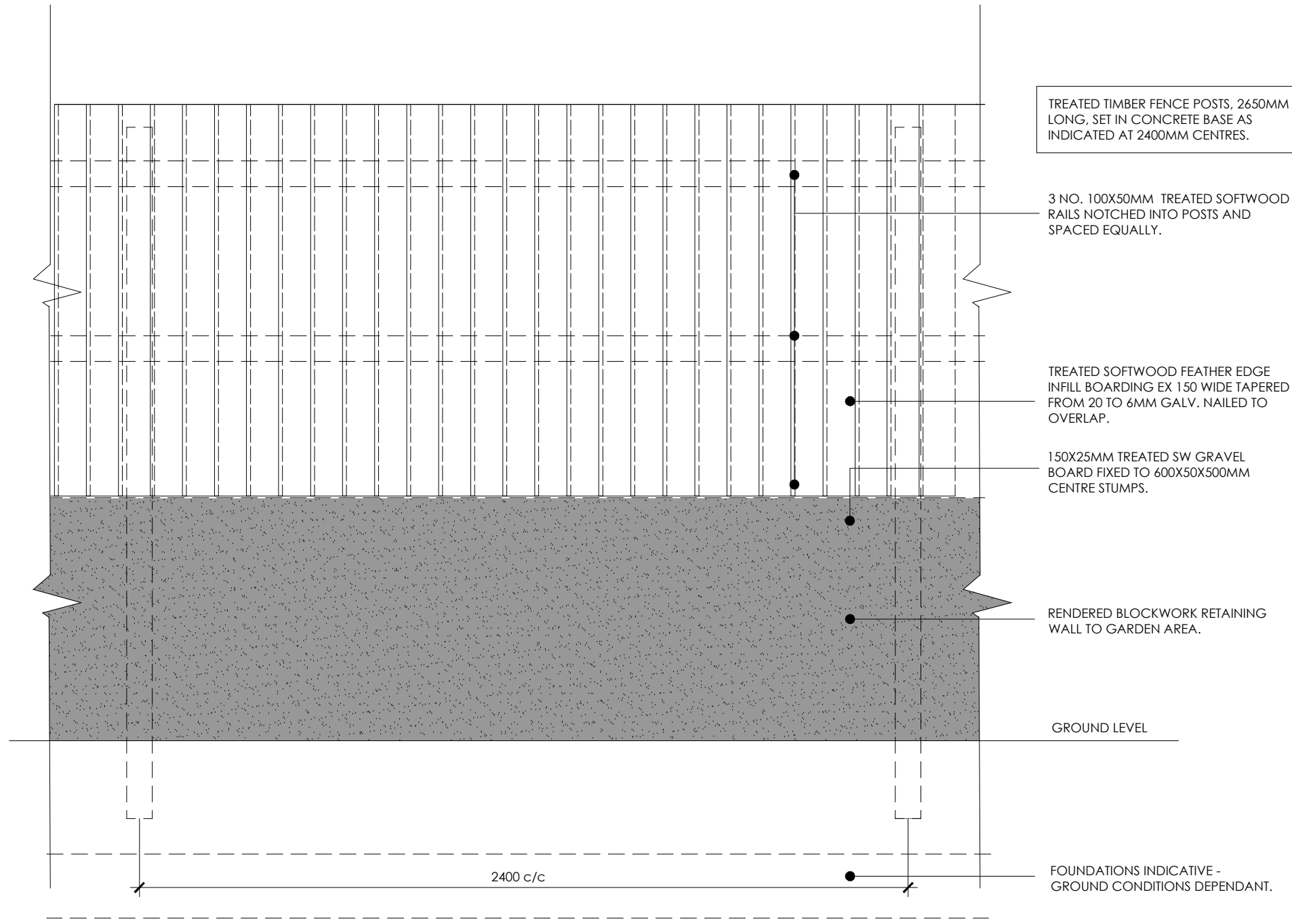
CLOSE BOARDED TIMBER FENCE _ 1800mm on retaining Wall
