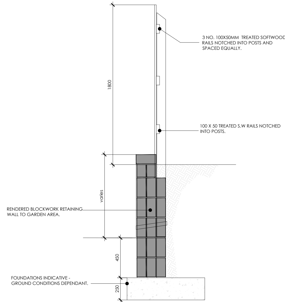
SECTION
