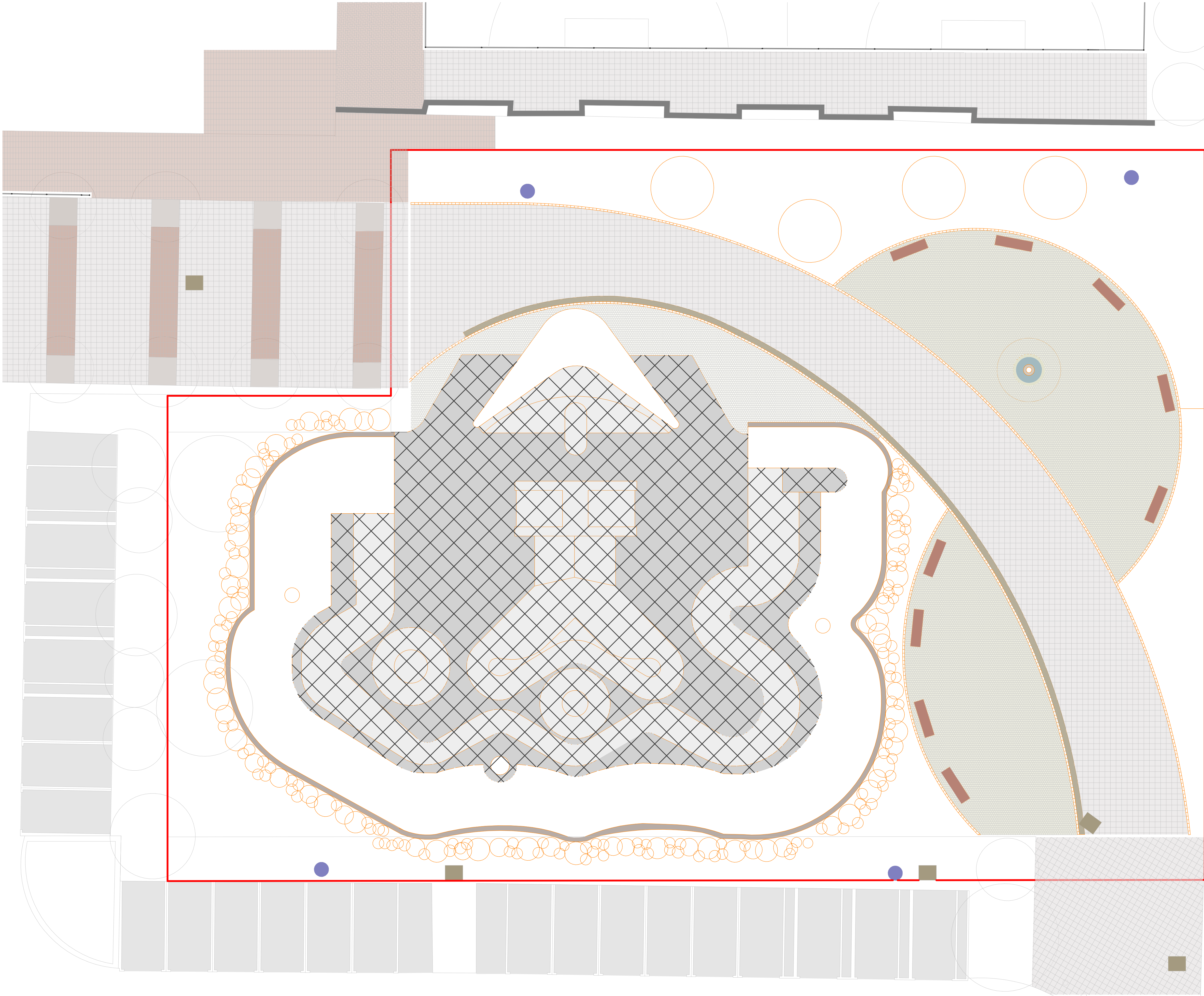
Hard Landscaping Layout 1 : 100
