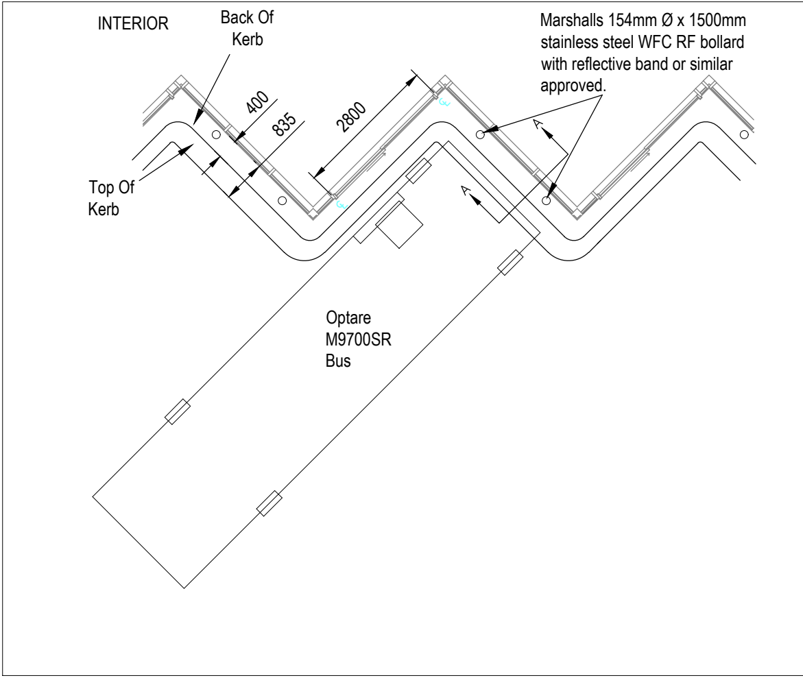
Detail of Parking Arrangement Optare M9700SR Bus Scale 1:100
