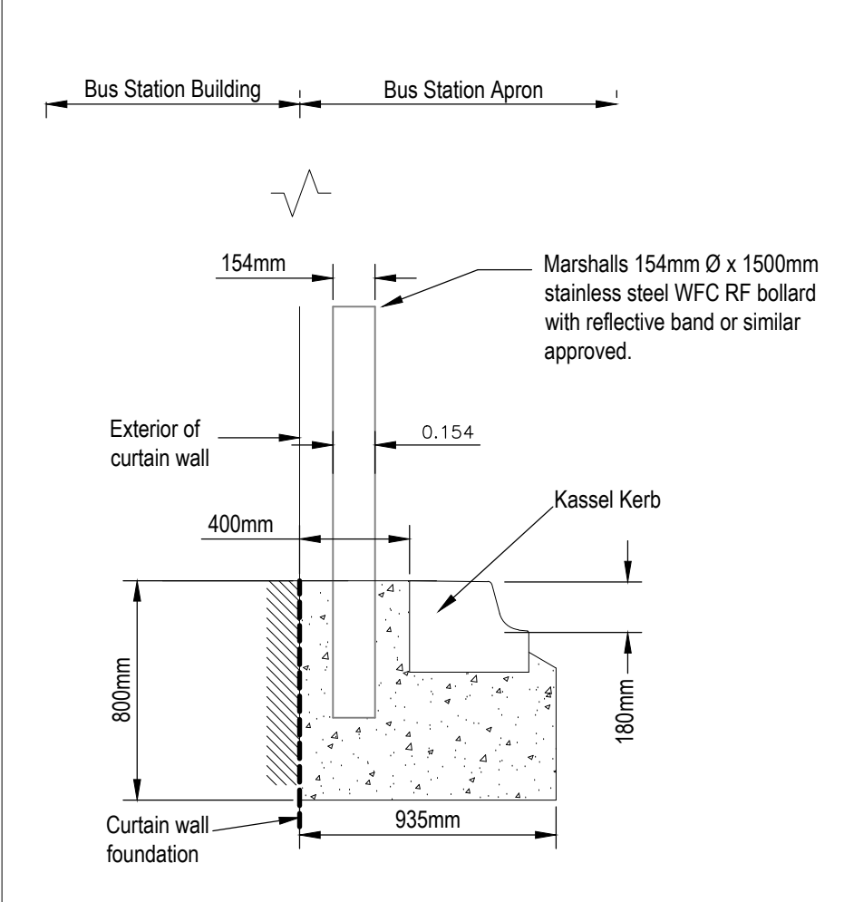
Cross Section A - A Detail of Marshalls Stainless Steel WFC RF Bollard or similar approved Scale 1:25
