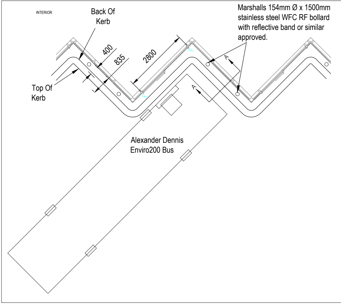
Detail of Parking Arrangement Alexander Dennis Enviro200 Bus Scale 1:100
