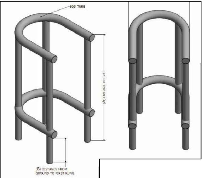
Detail A Street Lighting Column Protection Not to Scale
