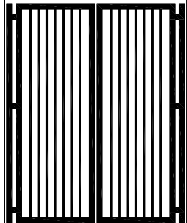
Replacement Refuse Store Gates - Elevation. 1:20@A1 Galvanised and powder coated (black) vertical bar bars. 18mm bars at 75mm centres. 50x50 perimeter box section frame with box section posts.
