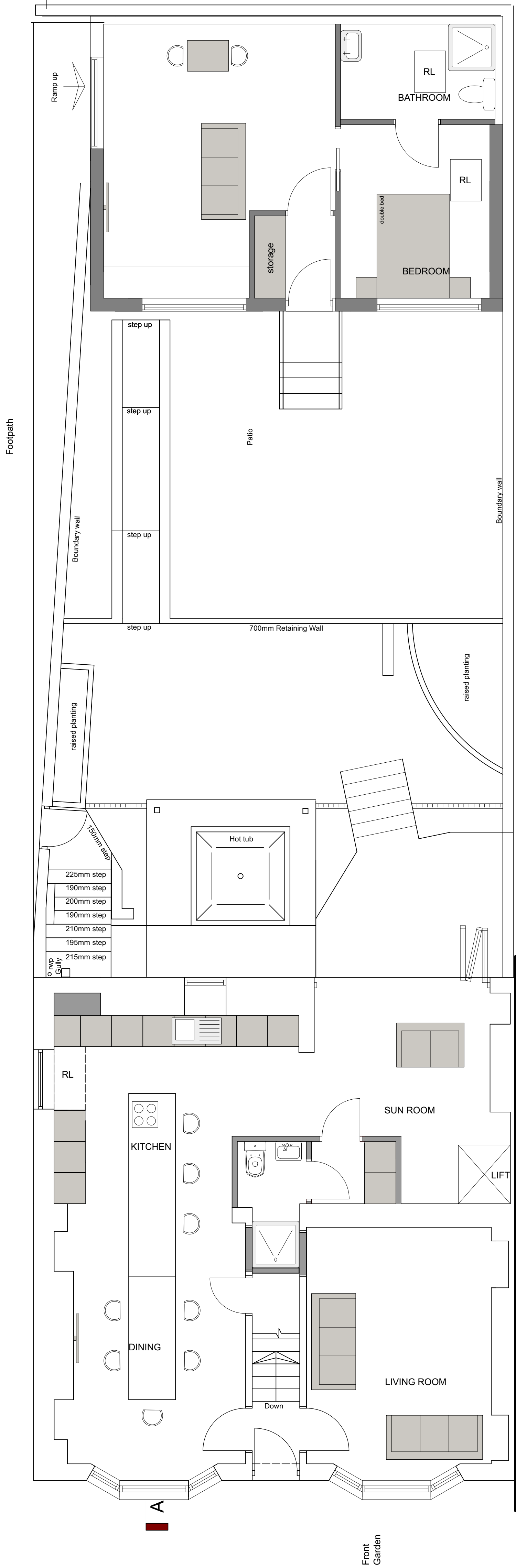
PROPOSED GROUND FLOOR
