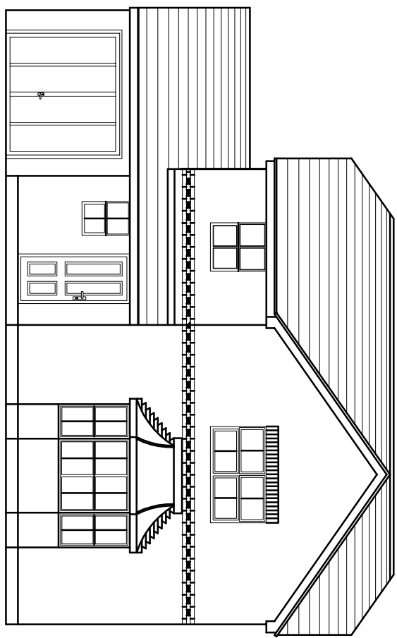
Front Elevation (North East)
