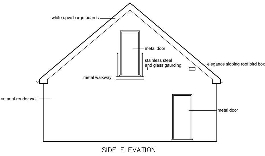
SIDE ELEVATION
