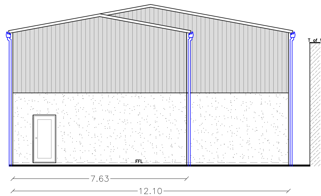
Proposed End Elevation 1:100
