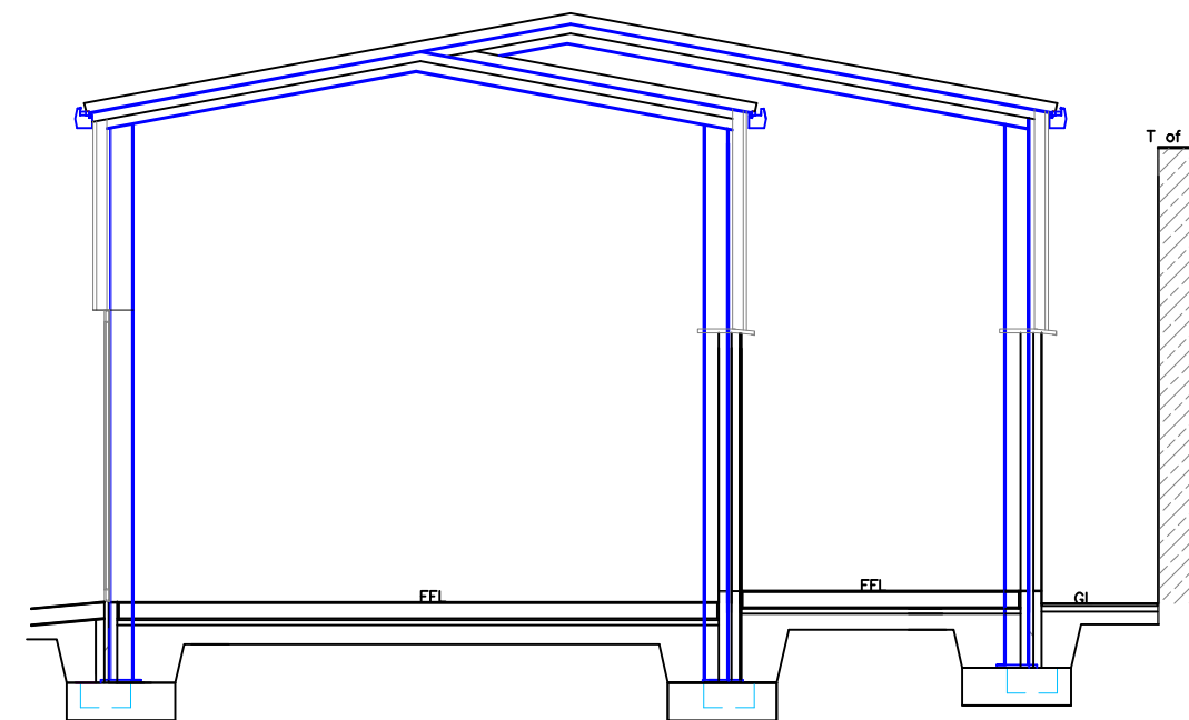
Proposed Section 1:100
