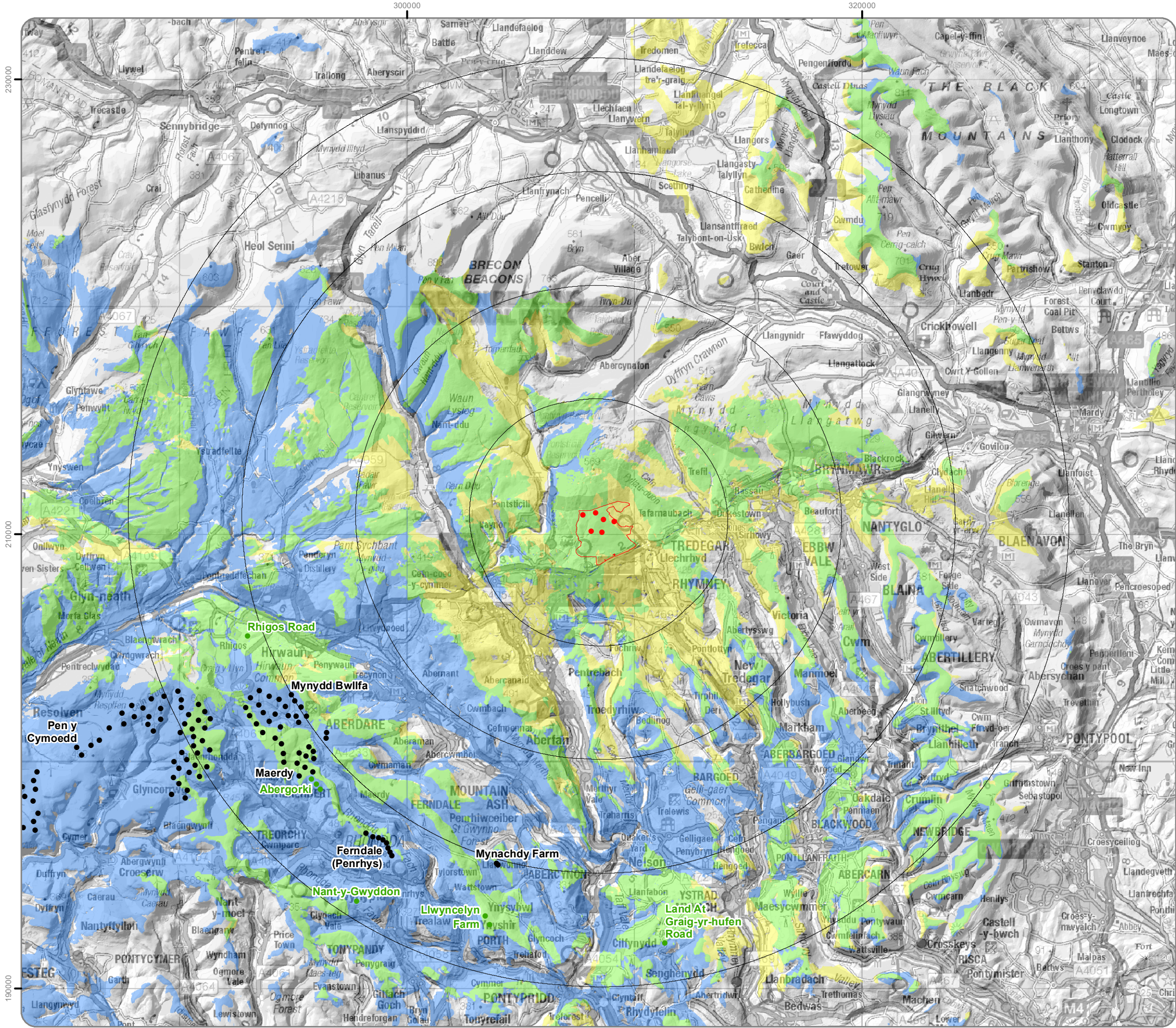
Figure 5.23f CZTV: Group 3 Operational and Consented Wind Energy Developments
