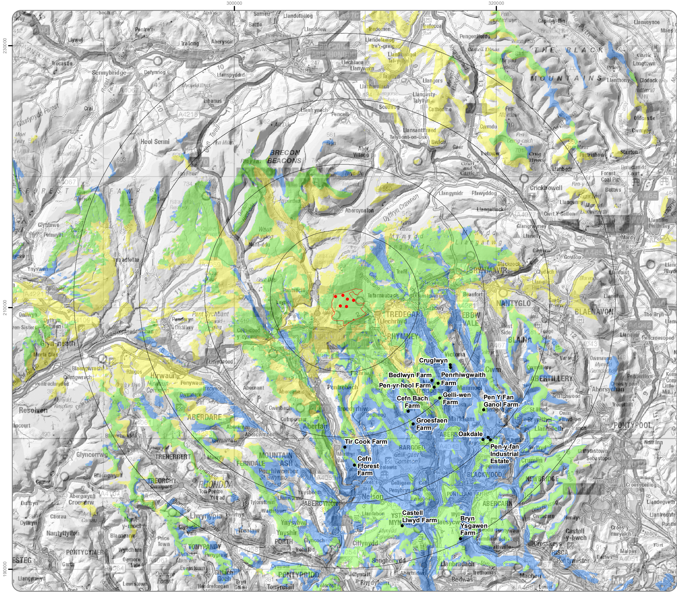
Figure 5.23c CZTV: Group 2 Operational Wind Energy Developments
