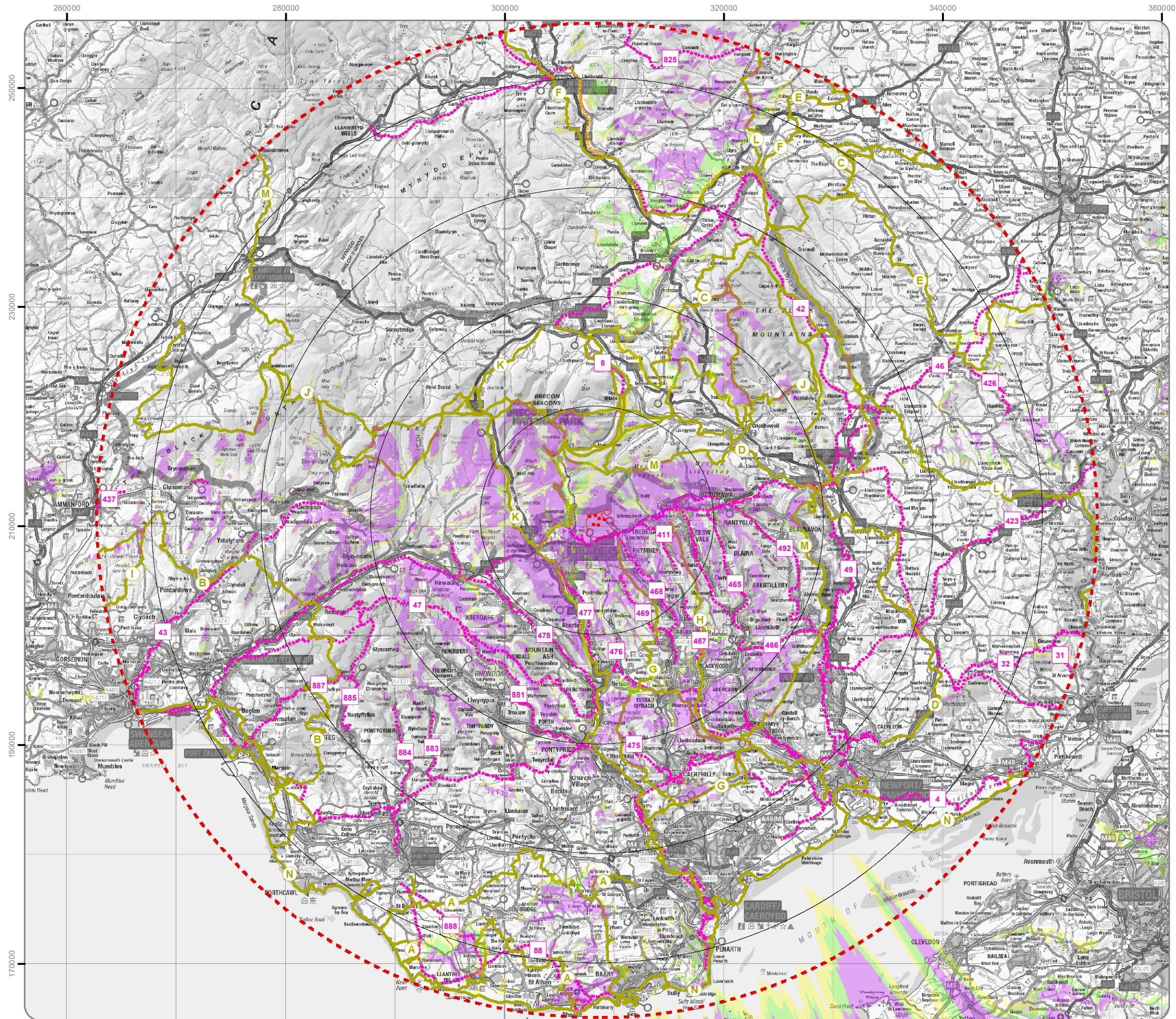
Figure 5.18 Principal Visual Receptors (Recreational Routes) and Blade Tip ZTV
