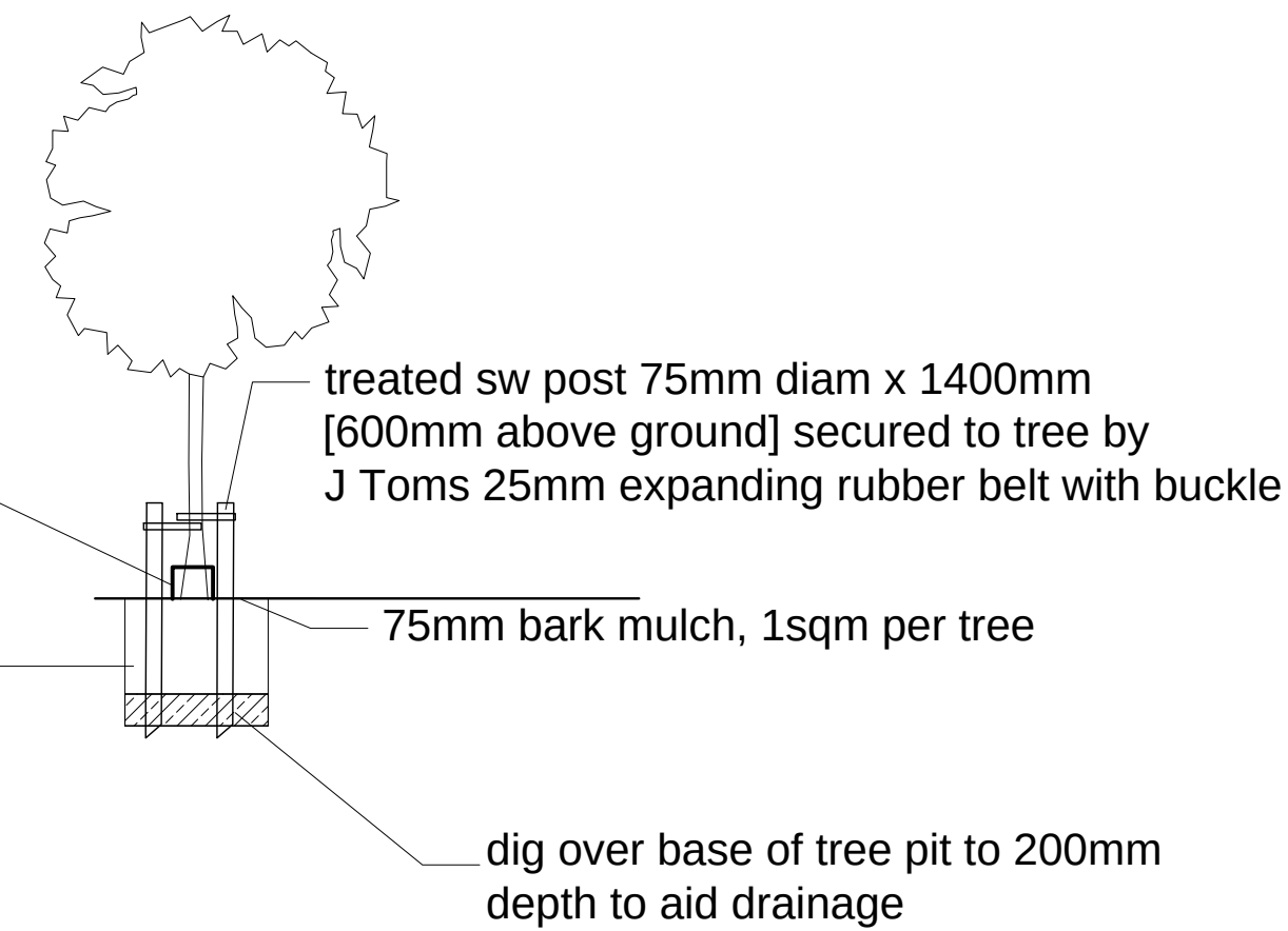
TREE PIT DETAIL @ 1: 50
