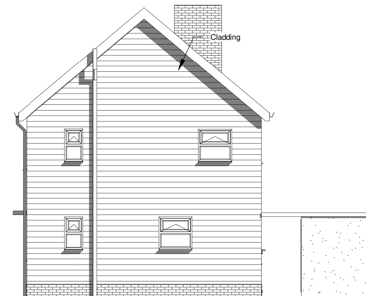
6 Existing Side 2 Elevation 1 : 100
