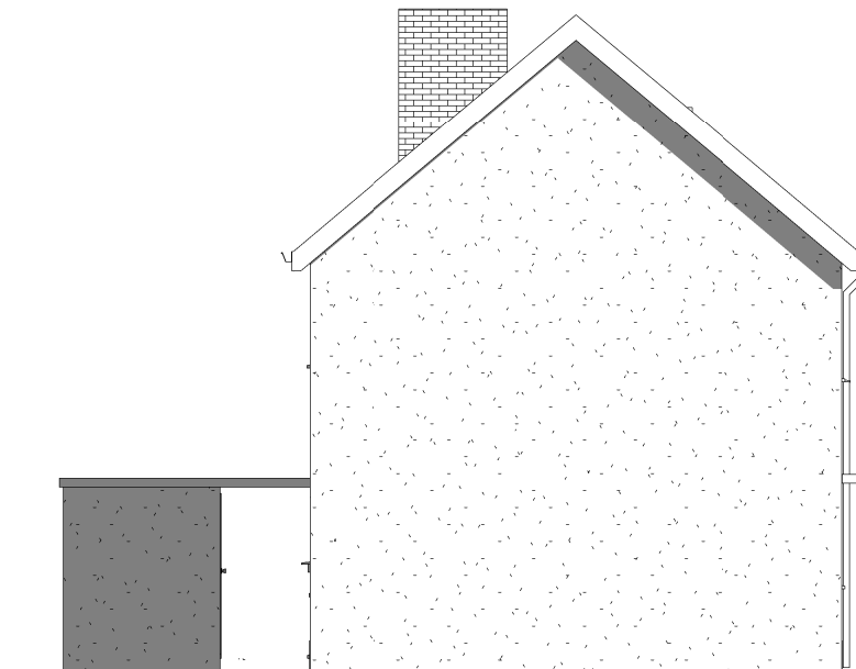
3 Existing Side 1 Elevation 1 : 100
