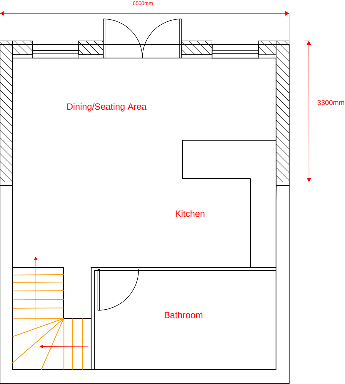
Proposed Lower Ground Floor Plan - 1:50
