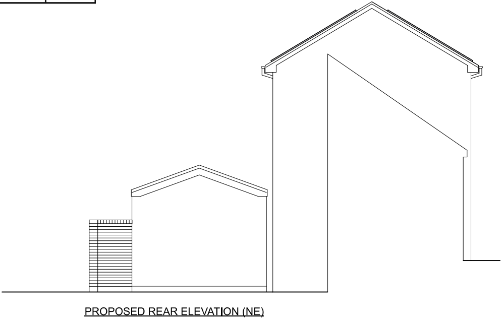
PROPOSED REAR ELEVATION (NE)
