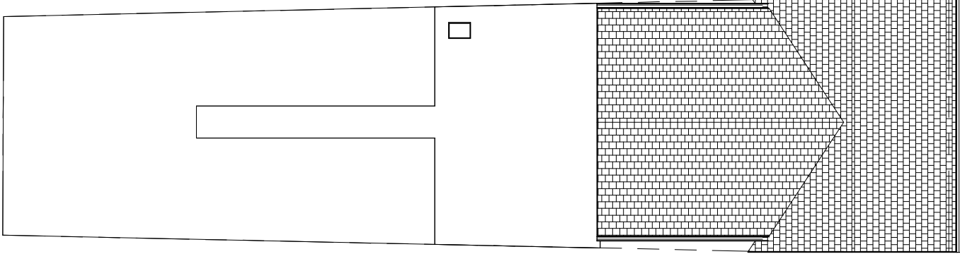
2 Proposed Site 1 : 100
