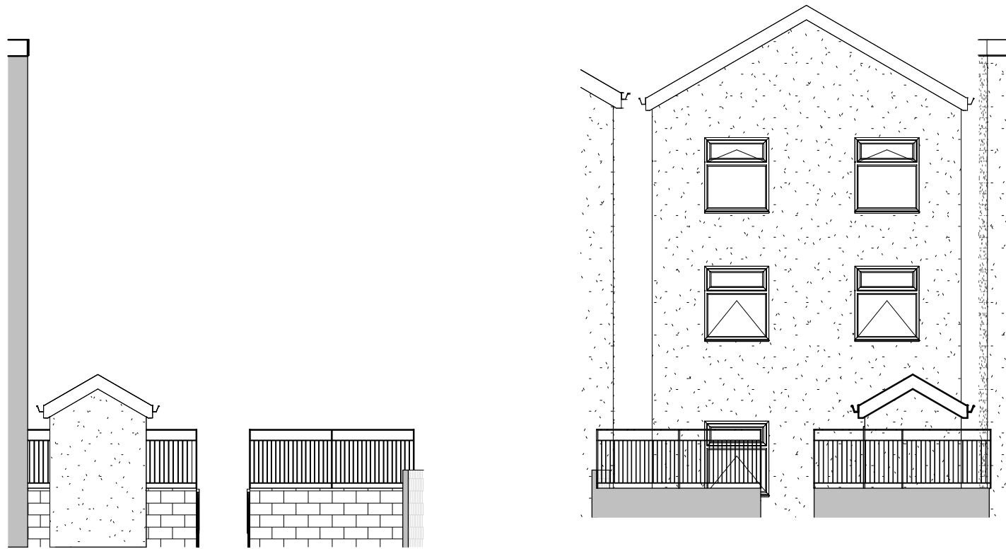
2 Rear Elevation 1 : 100
