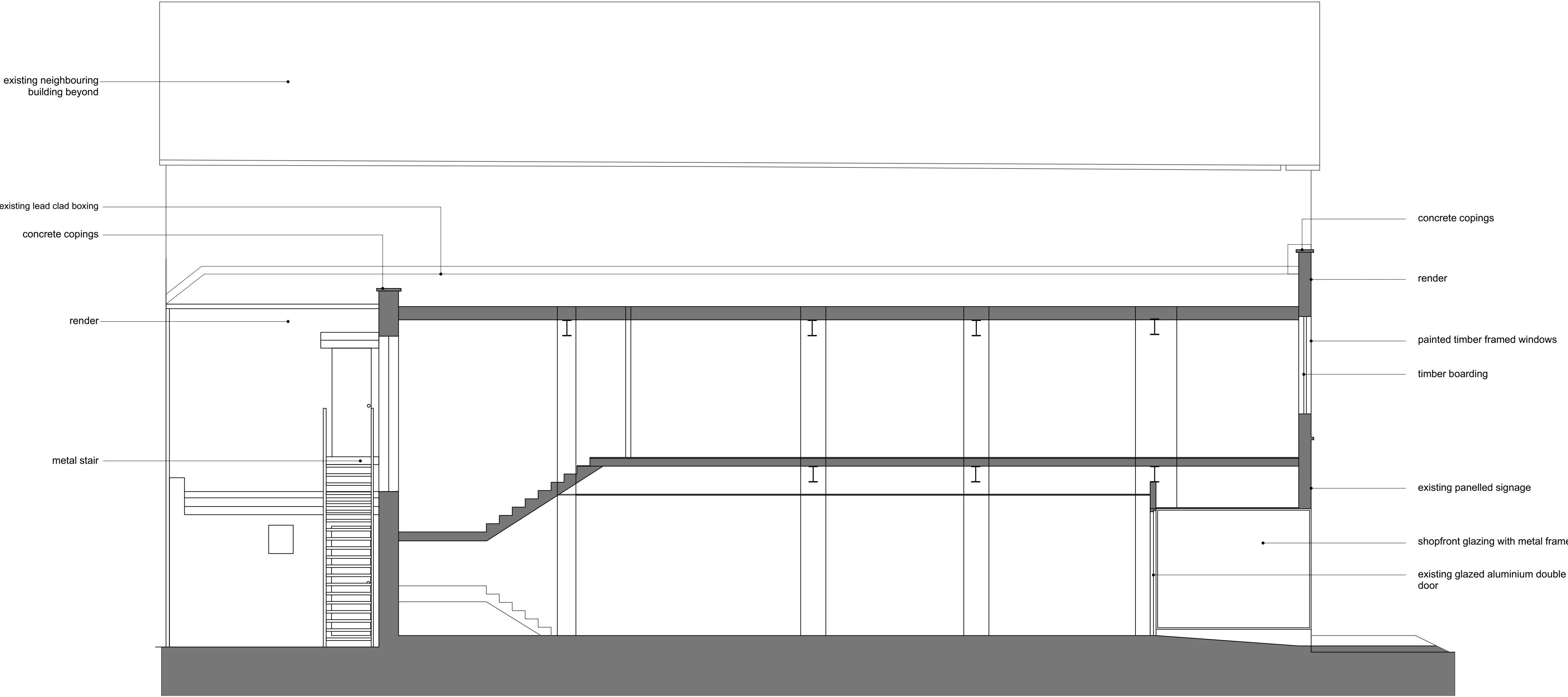
01 existing section
