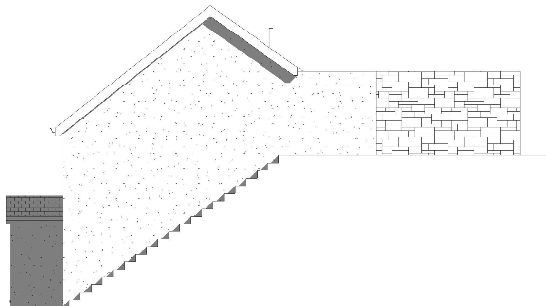
4 Existing Side 2 Elevation 1 : 100
