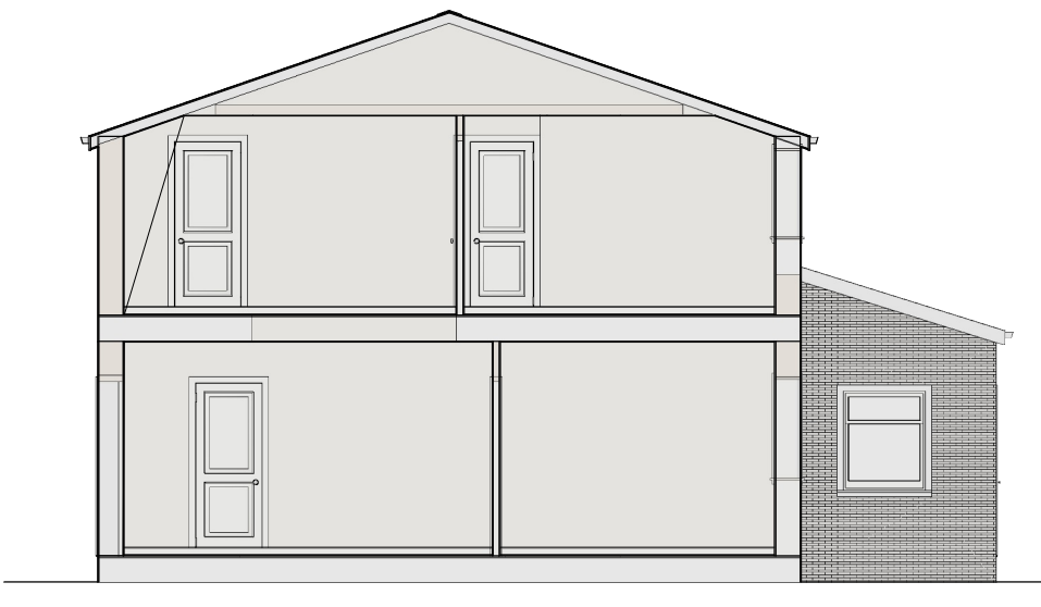
Existing second side elevation (section through)
