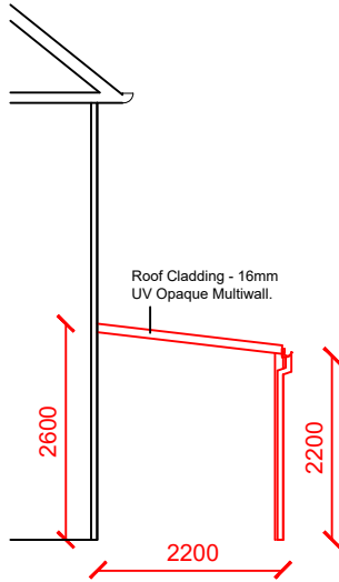
Side Elevation of Canopy
