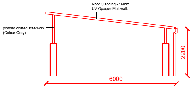
Side Elevation of Canopy
