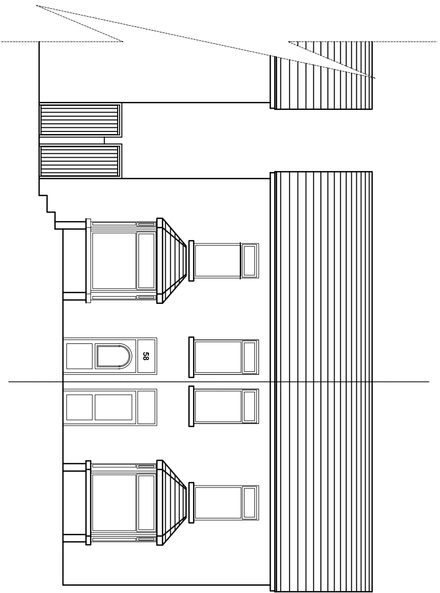
Front Elevation
