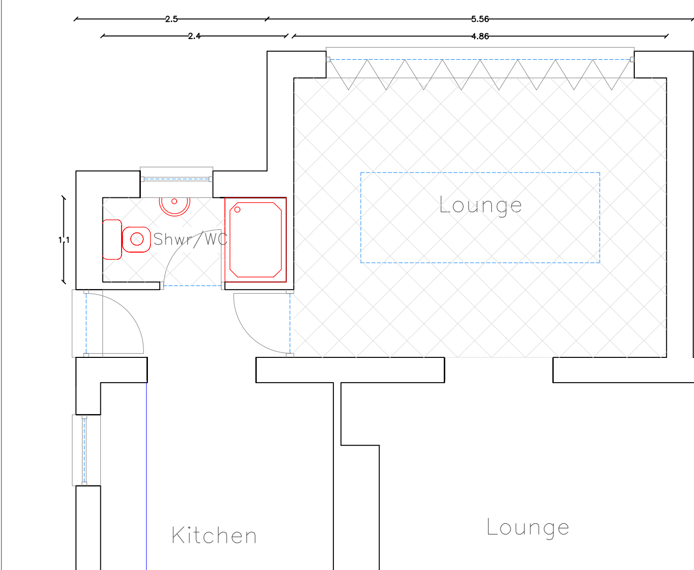
Proposed Extension Ground Floor Plan 1:50
