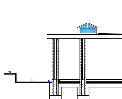
Proposed Section 1:100
