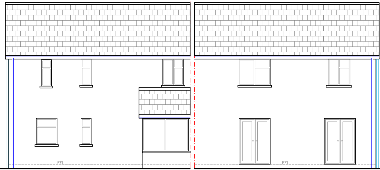
Existing Front Elevation 1:100 No Change
