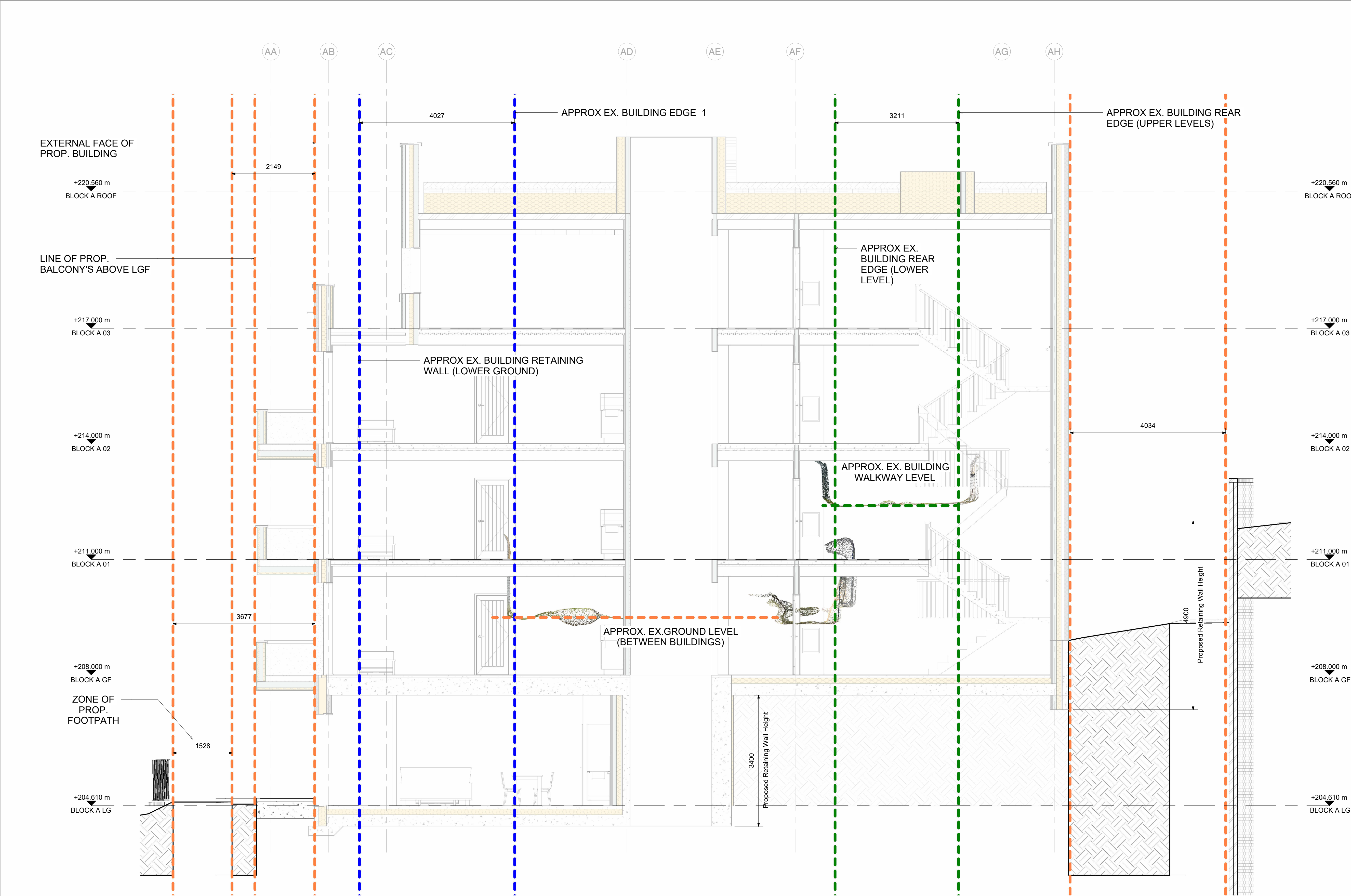
SECTION A - THROUGH BUILDING A & GARAGES 1 : 50
