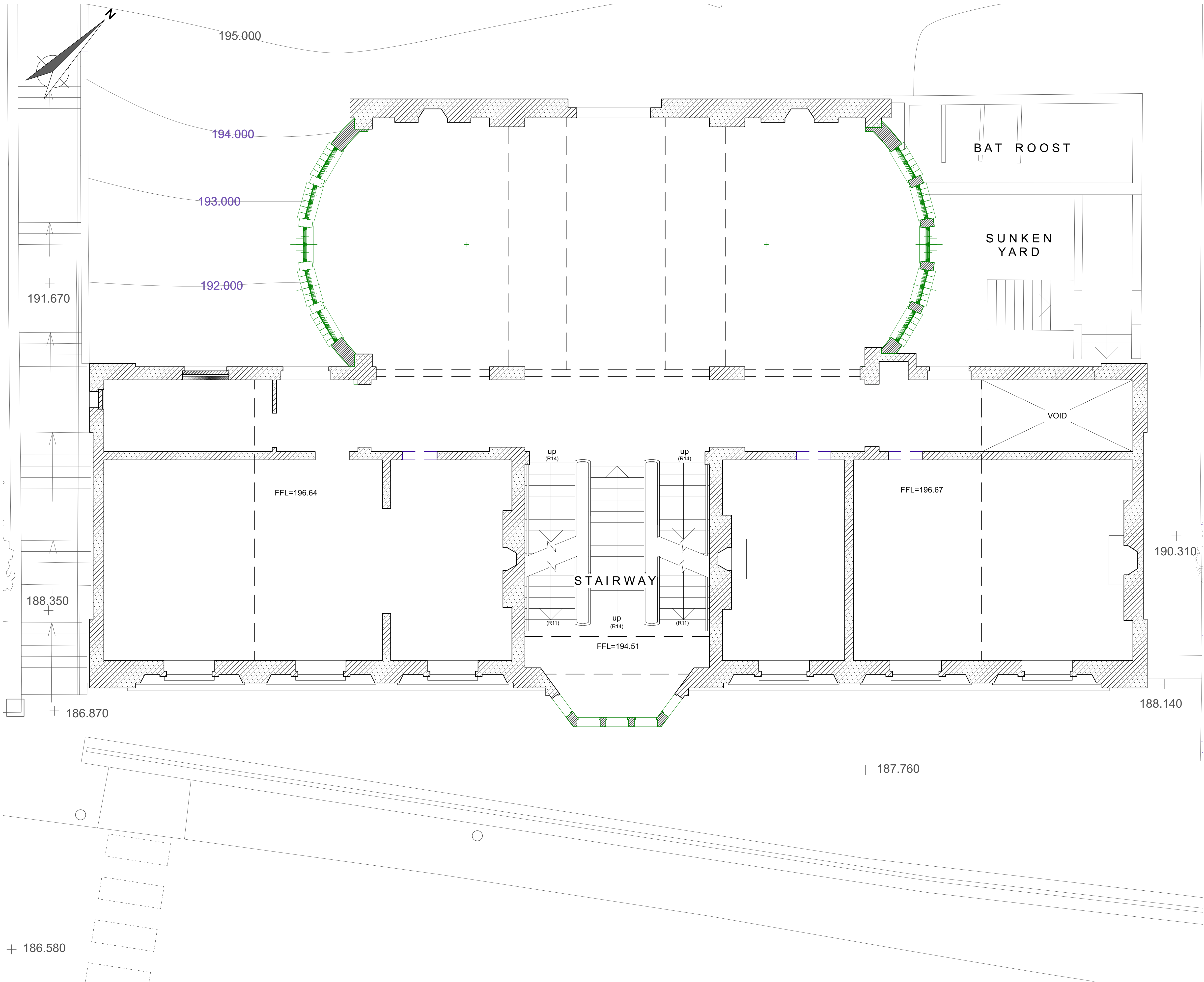
1 First Floor Demolition Plan Scale: 1:50
