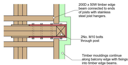
DETAIL 08 - PLAN VIEW OF BALUSTRADE POST TO BEAM CONNECTION SCALE 1:10
