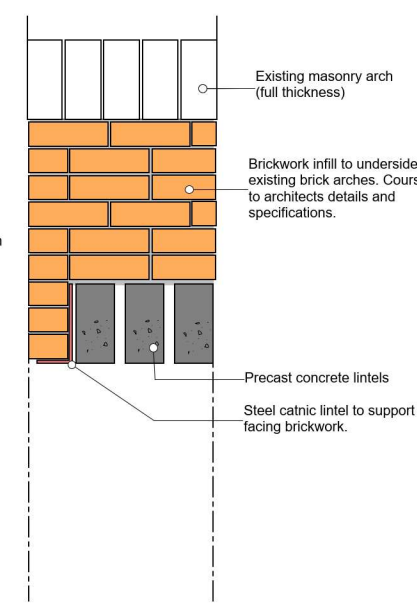
DETAIL 03 - PROPOSED OPENING AND WINDOW INFILL DETAIL SCALE 1:10
