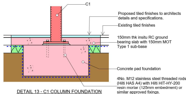
DETAIL 13 - C1 COLUMN FOUNDATION DETAIL IN BASEMENT
