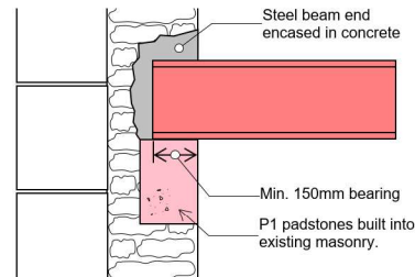
DETAIL 12 - TYPICAL STEEL BEAM TO EXISTING MASONRY CONNECTION SCALE 1:10
