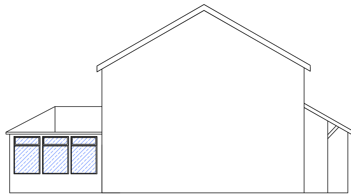
WEST SIDE ELEVATION EXISTING
