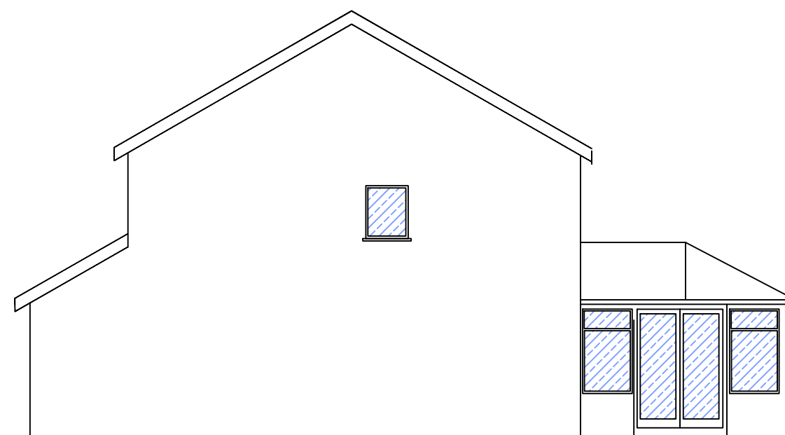
EAST SIDE ELEVATION PROPOSED
