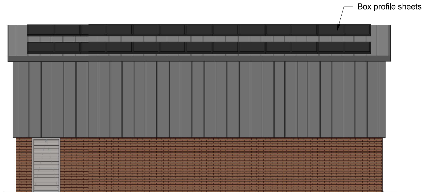
4 Proposed Side Elevation 1 : 100
