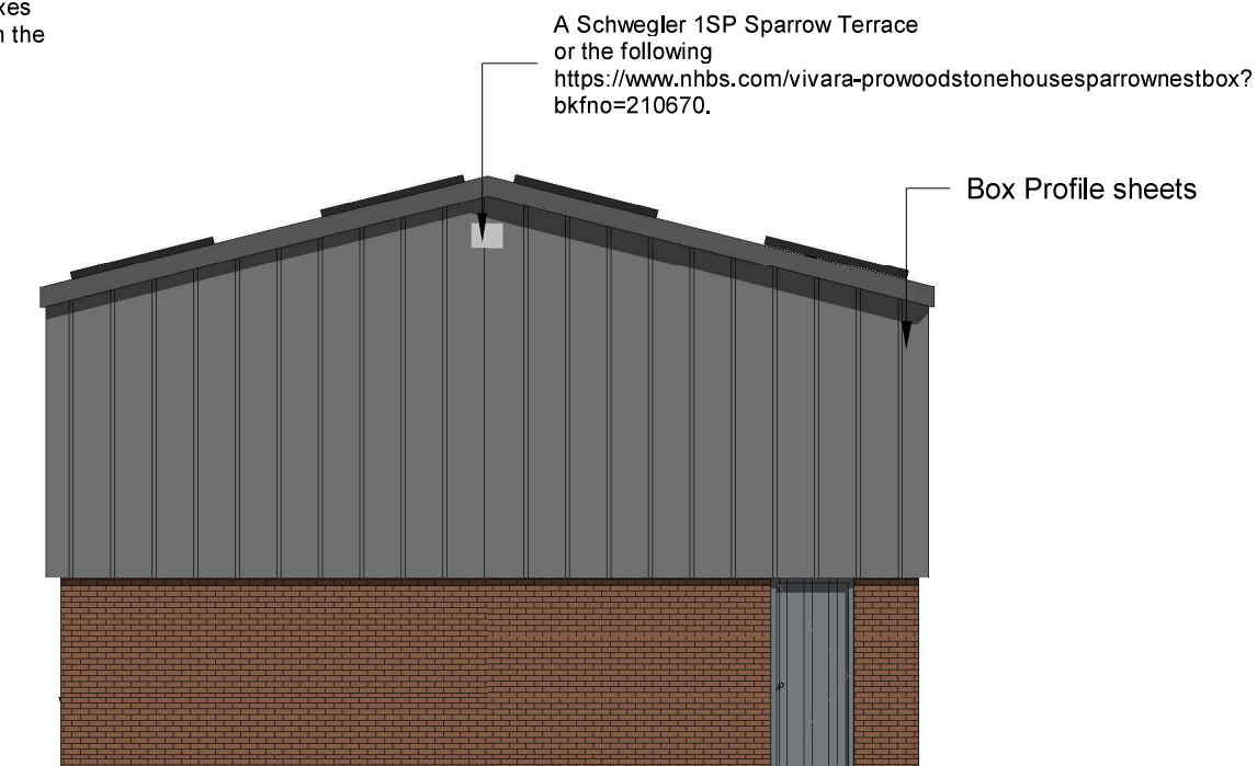
2 Proposed Rear Elevation 1 : 100
