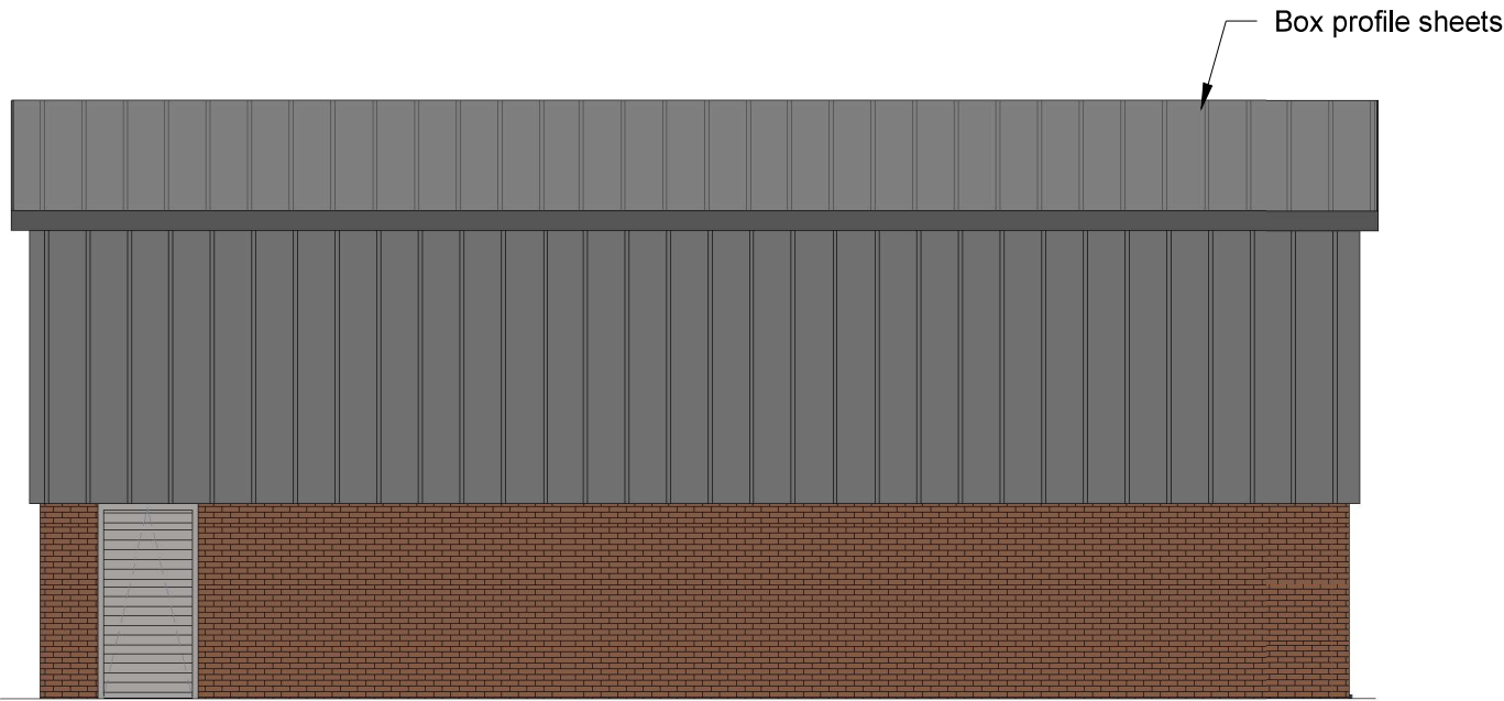
2 Existing Side Elevation 1 : 100
