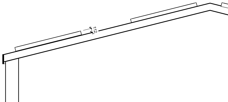
3 Proposed Section 1 : 50
