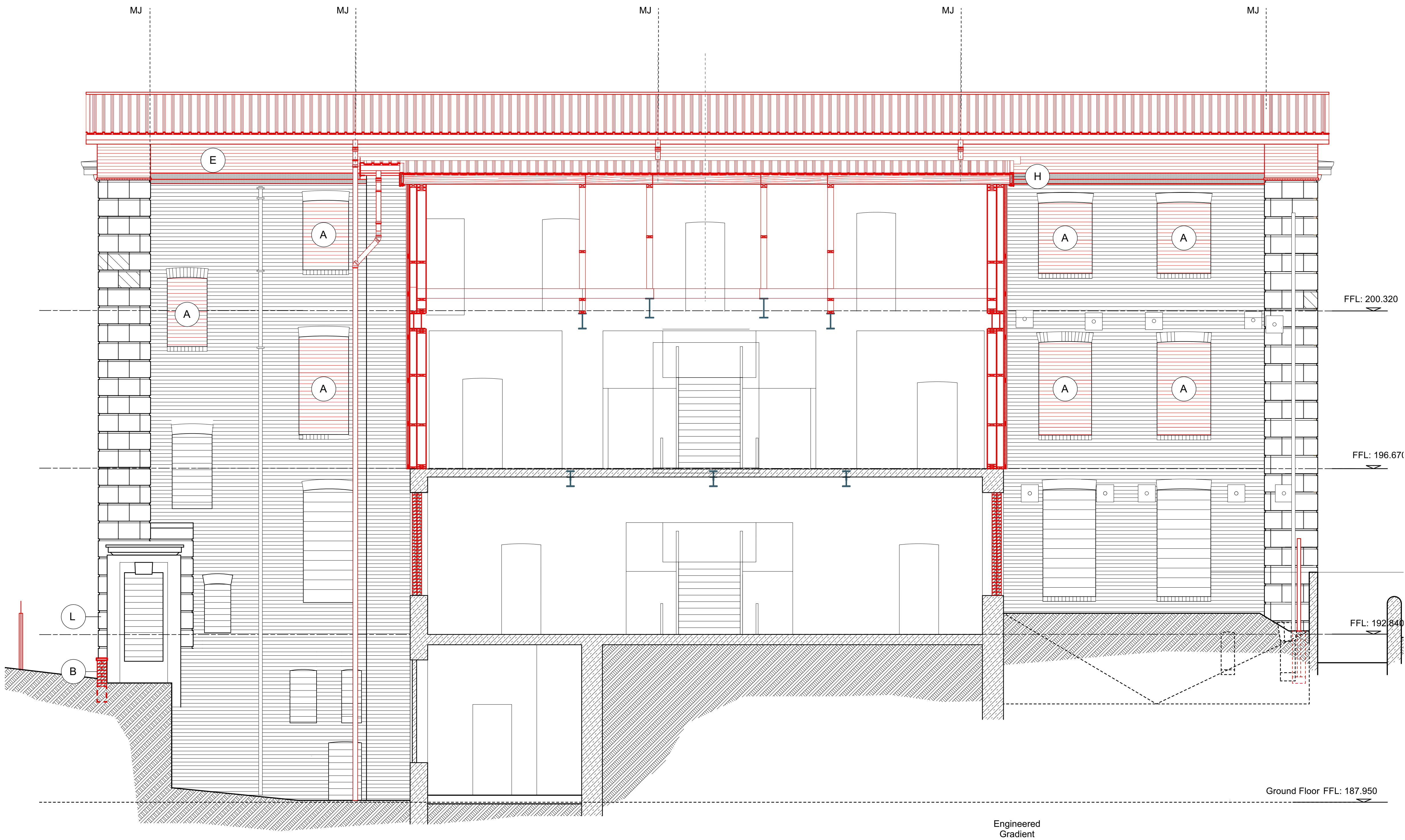
1 Proposed Long Section C-C Scale: 1:50
