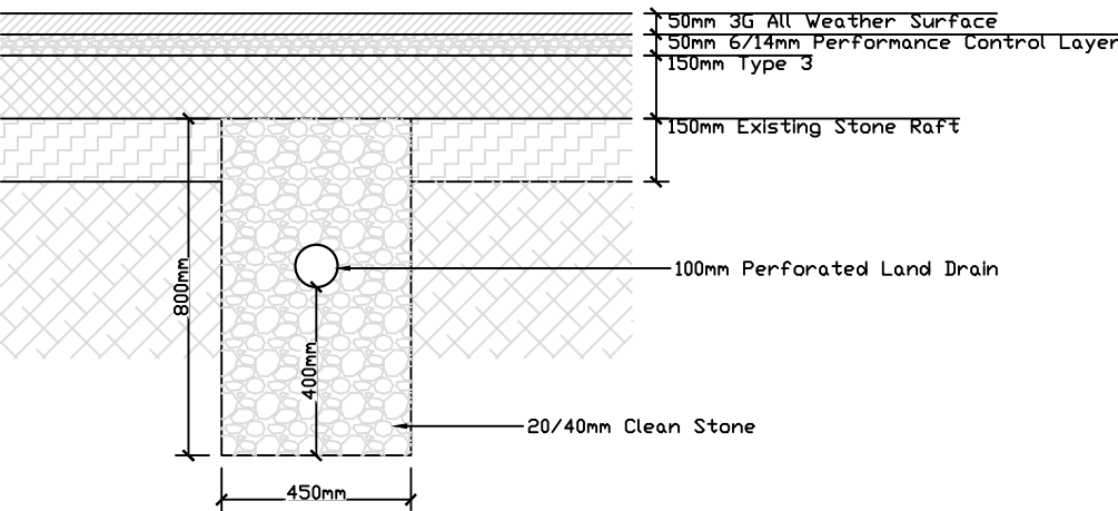
NEW Drainage Lateral Type C (NO Baffle)
