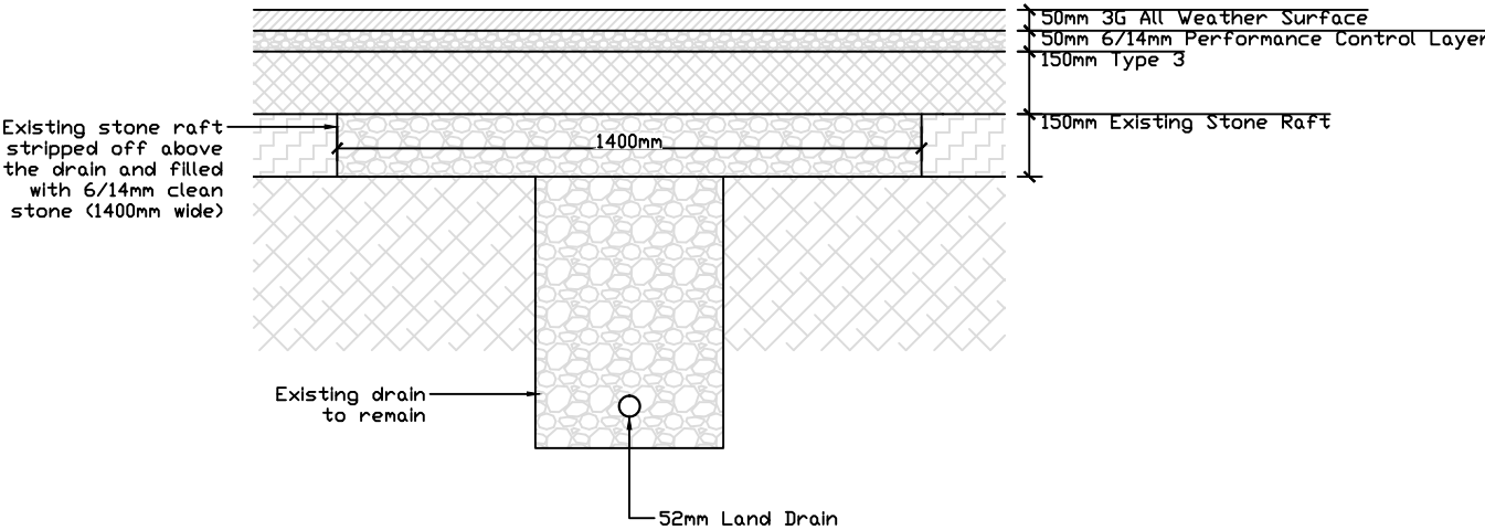
Upgrade to Existing Drainage Lateral Type A
