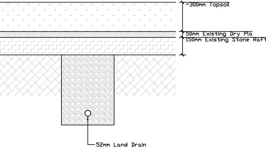
Existing Drainage Lateral TYPE X
