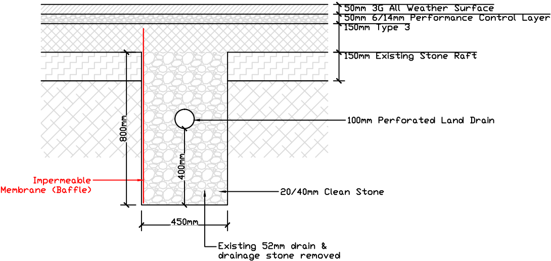
NEW Drainage Lateral Type B1/2 (BAFFLE)
