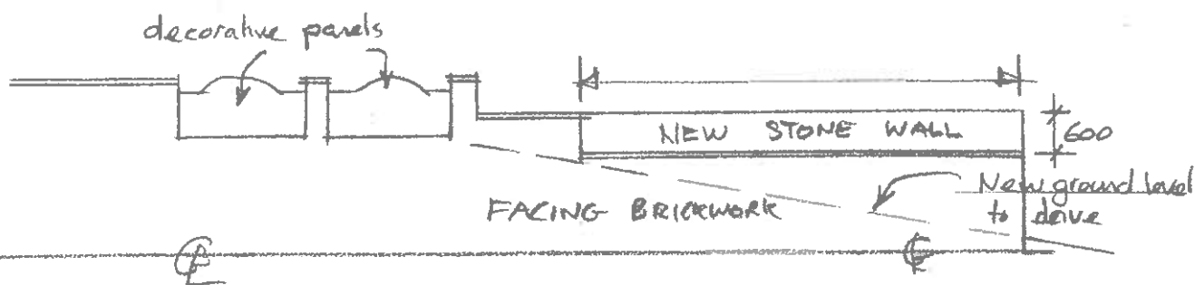
PROPOSED ELEVATION FROM TY CROESO
