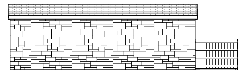
4 Proposed side 1 Elevation 1 : 100
