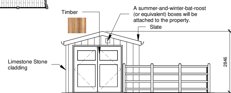
2 Proposed Front Elevation 1 : 100
