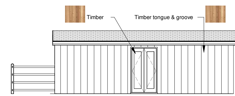
5 Proposed side 2 Elevation 1 : 100
