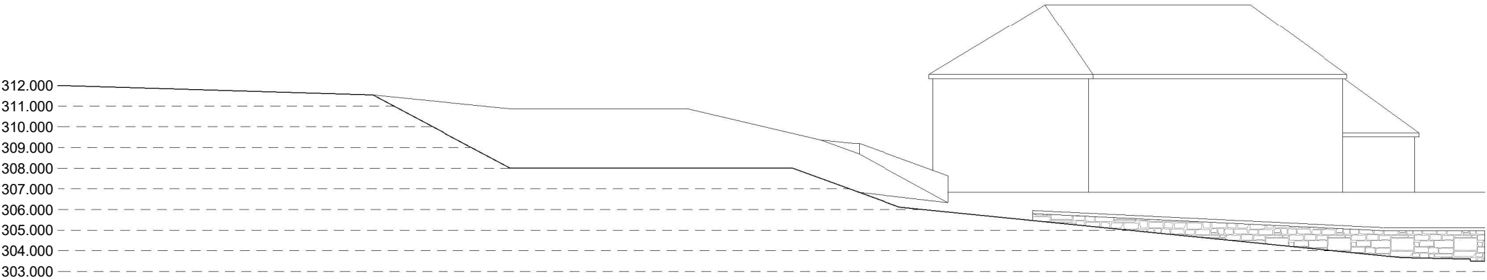
Section Along Existing Retaining Wall
