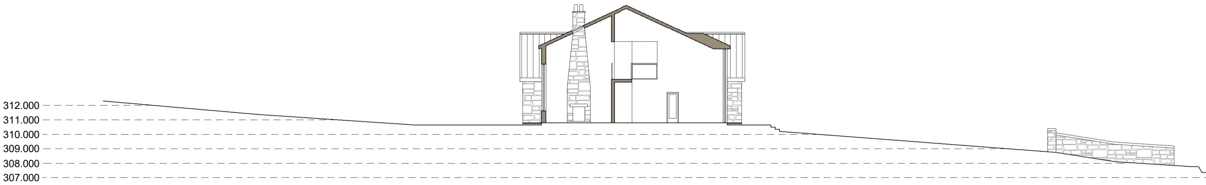
Section Through Dwelling
