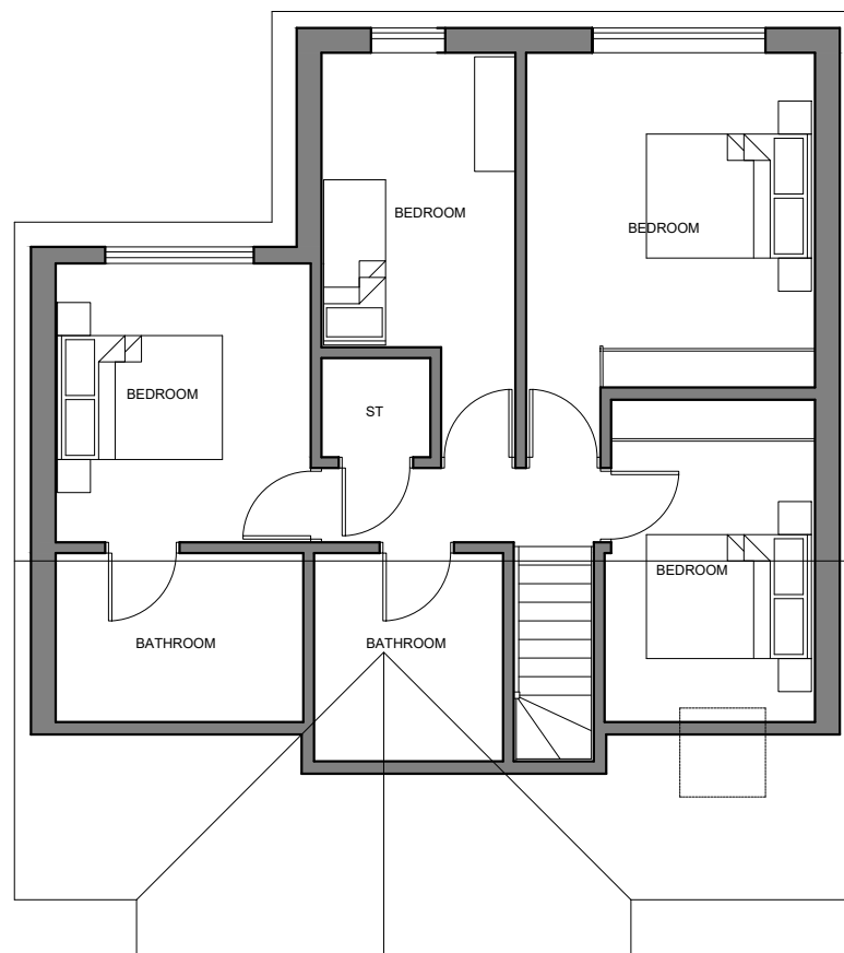
PROPOSED FIRST FLOOR LAYOUT
