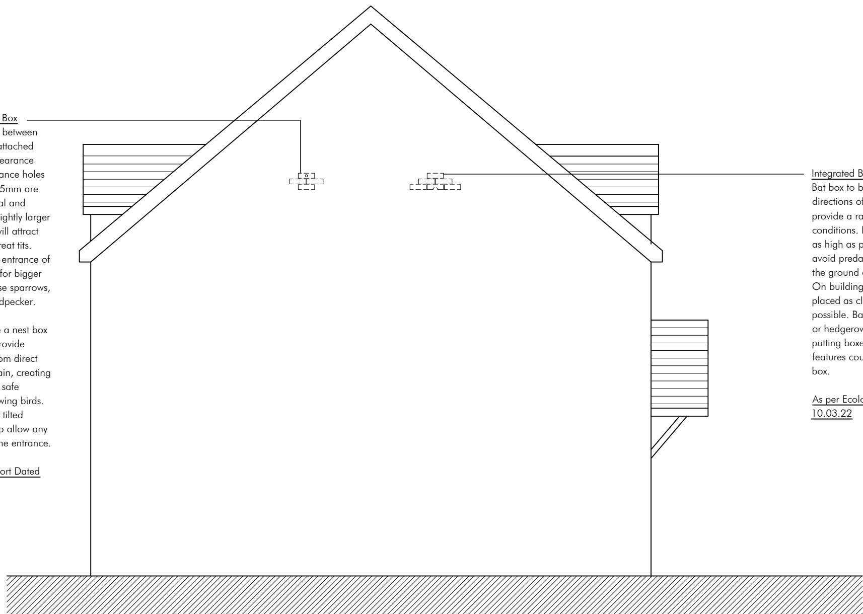
PROPOSED SIDE (NORTH) ELEVATION 1:50
