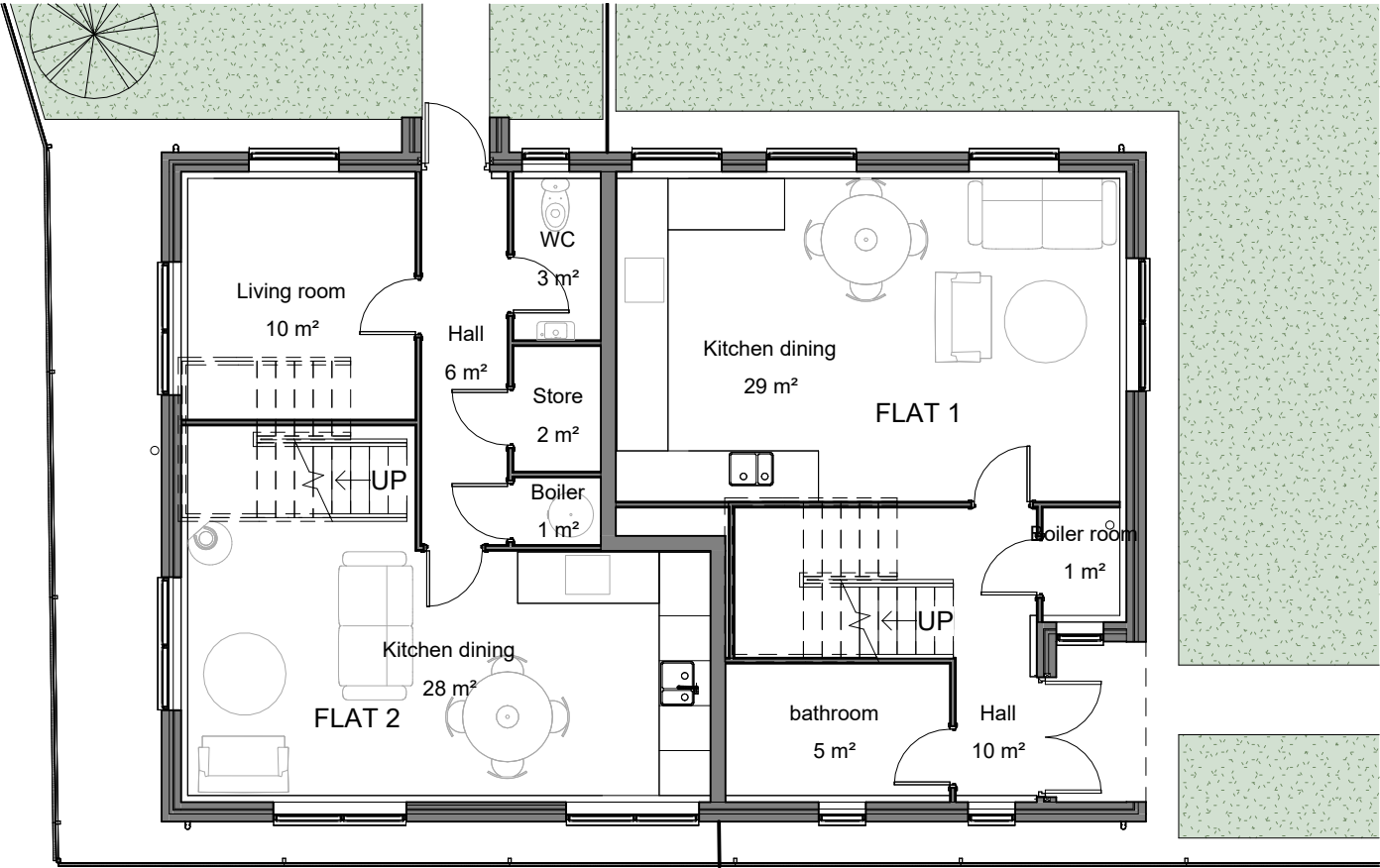
Ground Floor Proposed ( 1 : 100)
