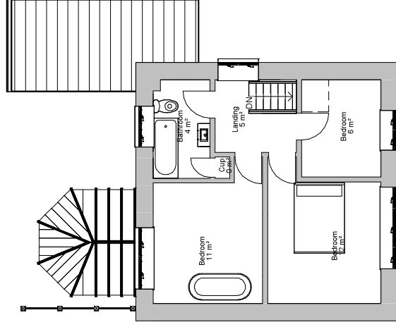
2 Existing First Floor 1 : 100
