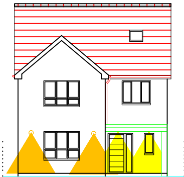
FRONT ELEVATION Scale 1 : 100
