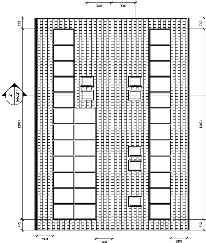
1 Proposed Roof Plan 1 : 100
