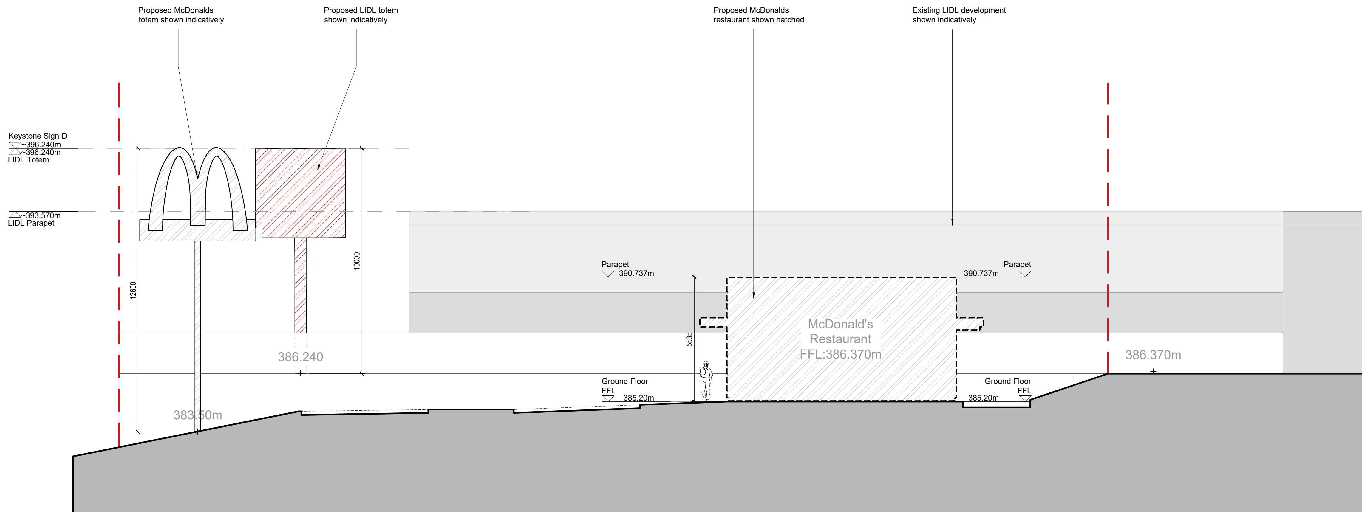
Proposed Site Section A Scale 1:100
