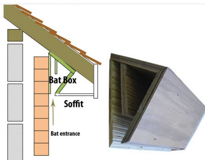
Figure MP6 Bat roost soffit-boxes to be provided at each of the four corners of the new house. This box is marketed by Wildcare Nationwide Ecology Supplies
