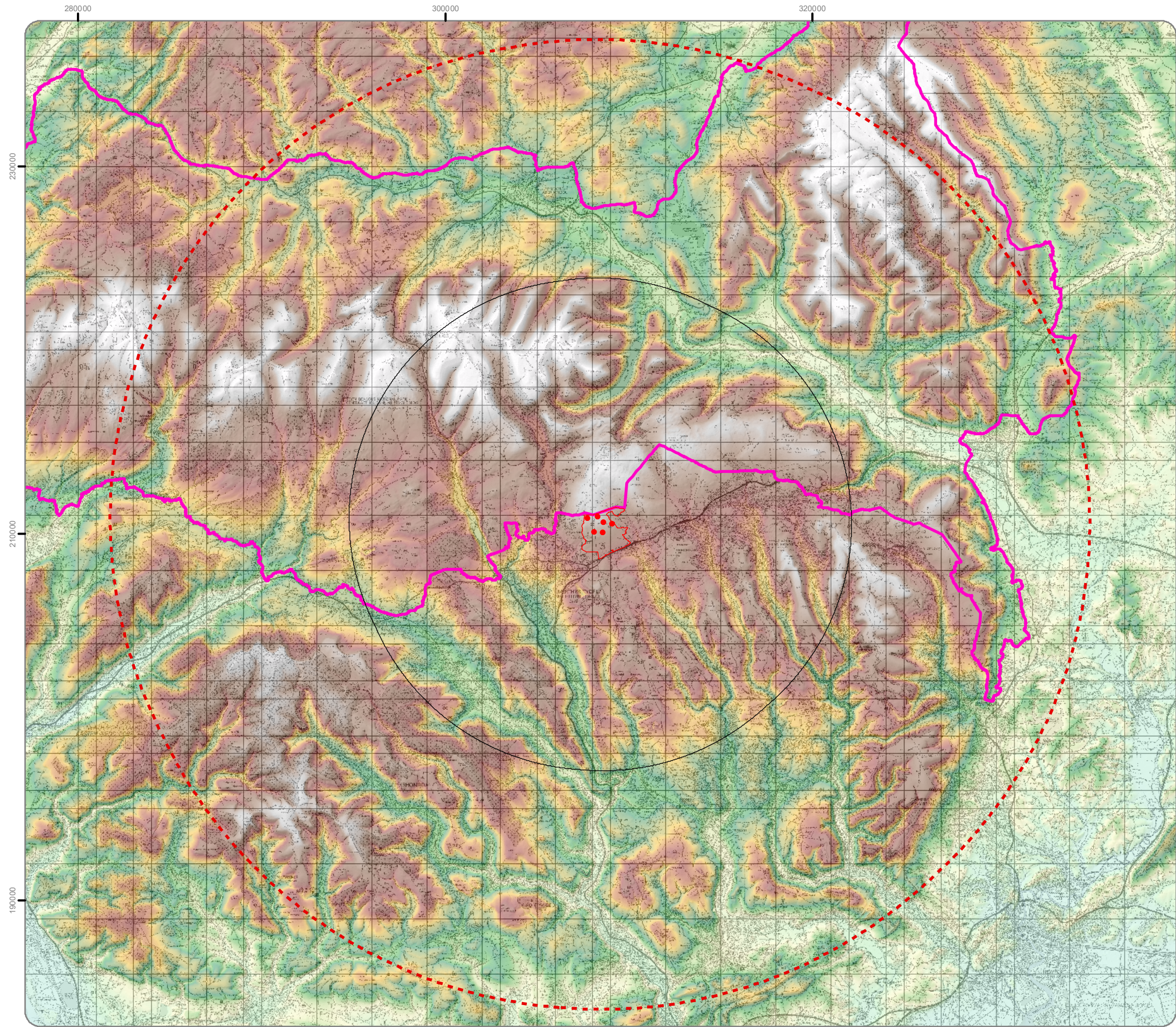
Figure 5.2 Landform
