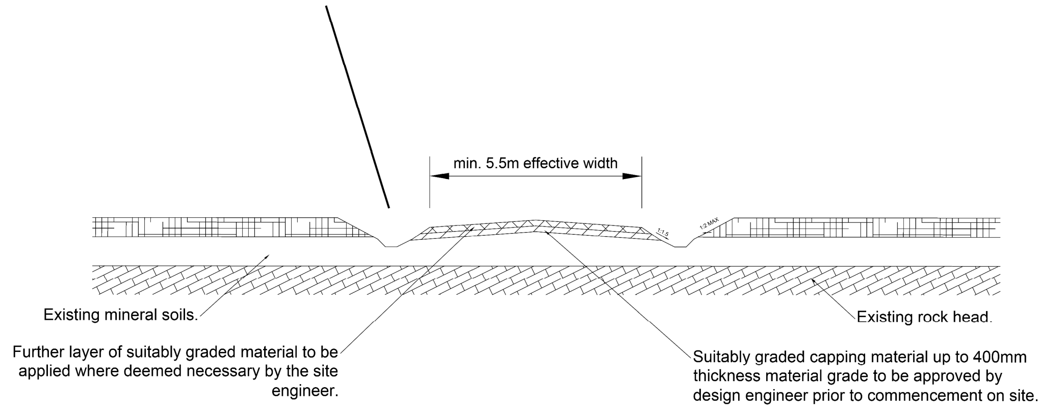
TYPICAL TRACK FORMATION ON OVERBURDEN SOIL
